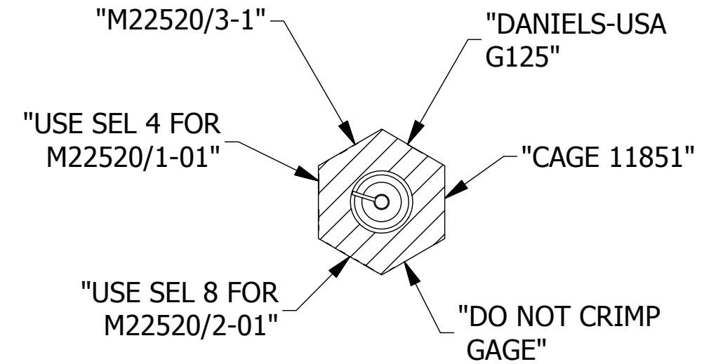
SECTION X-X
